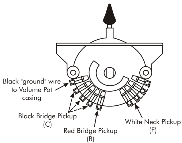
"Ground Side" Wafer Layout
