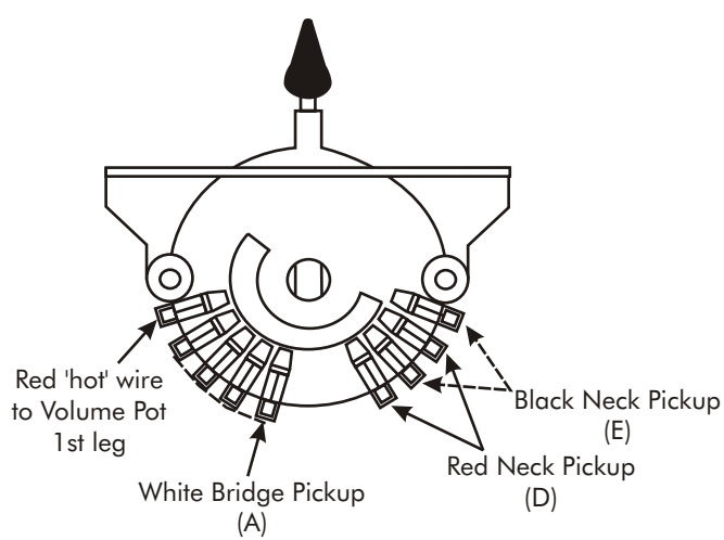
"Hot Side" Wafer Layout
